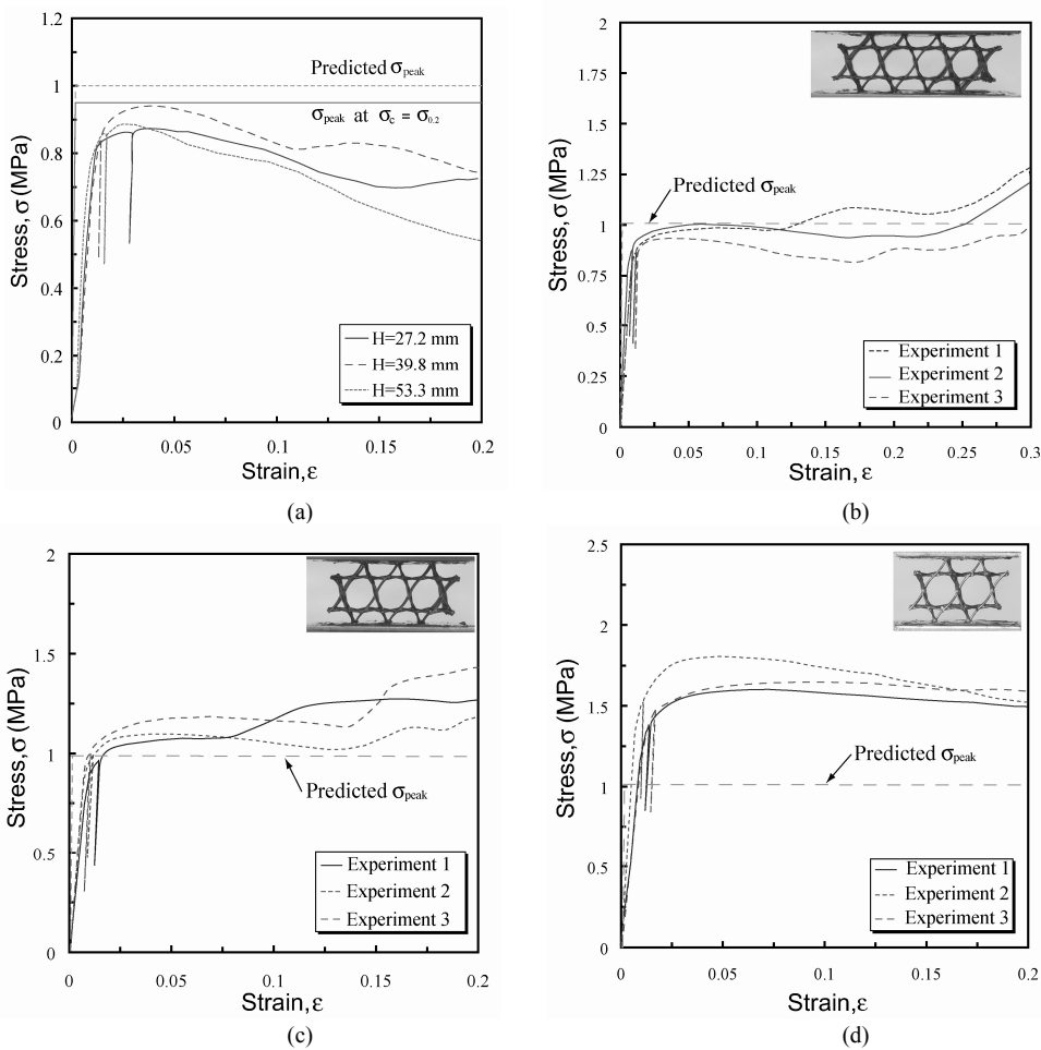
Fig. 3. (a) Representative stress-strain curves of specimens with different heights [8], and measured curves of the specimen with (b) L_e=48.6\text{mm} , (c) L_e=32.4\text{mm} and (d) L_e=24.3\text{mm} plotted together with the analytically predicted peak stress.
